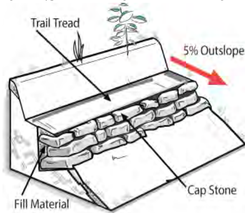
Figure 6: Typical MPOS Design for Natural Retaining Walls
