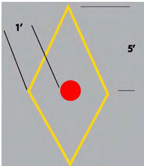
Figure 14: Typical Striping around Bollard
