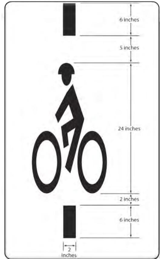
Recommended loop detector marking design.
